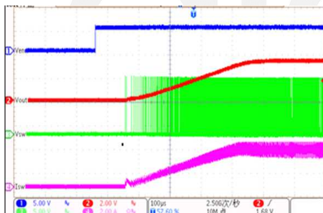
Start up from Enable ( V_{IN}=12V, V_{OUT}=3.3V, Load=1\Omega )
