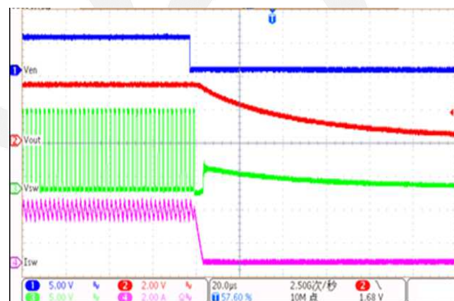
Shut down from Enable ( V_{IN}=12V, V_{OUT}=3.3V, Load=1\Omega )
