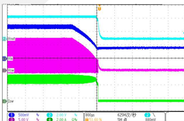
Shut down from VIN ( V_{IN}=12V, V_{OUT}=3.3V, Load=1\Omega )
