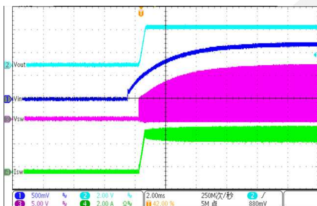
Start up from VIN ( V_{IN}=12V, V_{OUT}=3.3V, Load=1\Omega )
