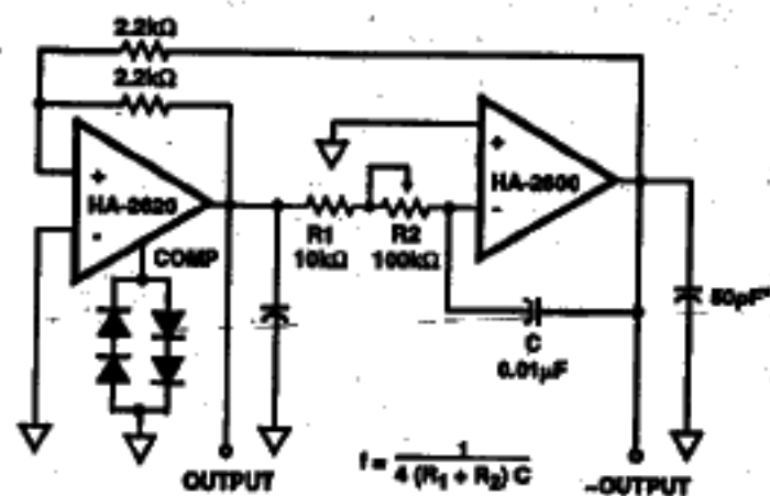
FIGURE 11. FUNCTION GENERATOR
