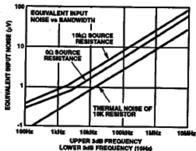
FIGURE 2. BROADBAND NOISE CHARACTERISTICS
