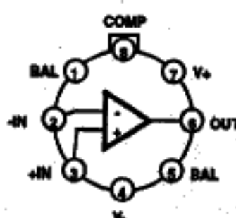
HA-2620, HA-2622, HA-2625 (CAN) TOP VIEW
