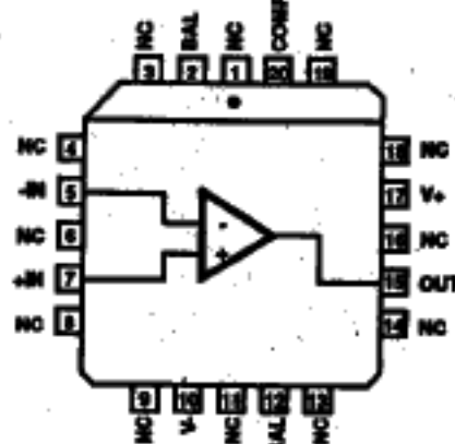
HA-2625, (PLCC) TOP VIEW
