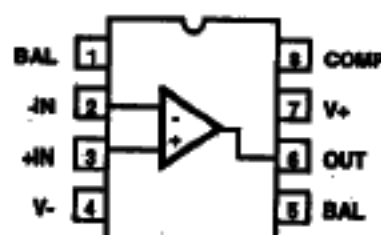
HA-2620/22 (CDIP) HA-2625 (CDIP, PDIP, SOIC) TOP VIEW
