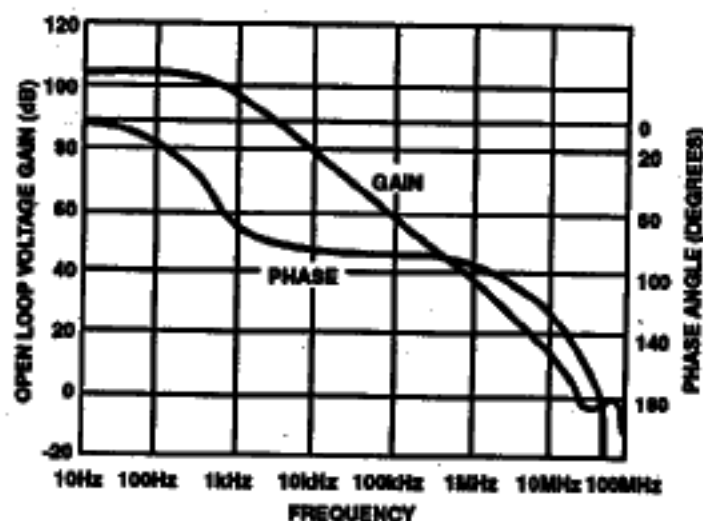
FIGURE 3. OPEN LOOP FREQUENCY AND PHASE RESPONSE
