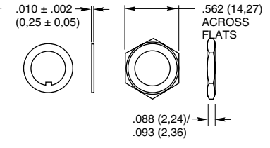
Keyed Washer Hex Nut
