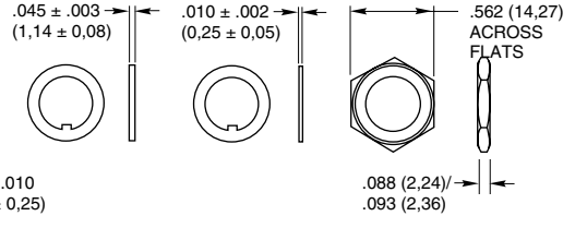
FIGURE C: Seal, Keyed Washer, Hex Nut
