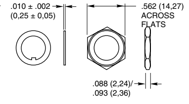
Keyed Washer
