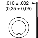
Keyed Washer
