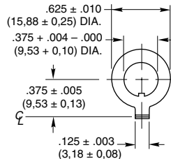
Non-Turn Washer
