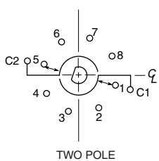
TWO POLE
