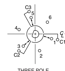
THREE POLE
