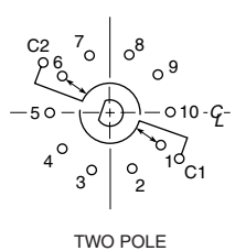
TWO POLE
