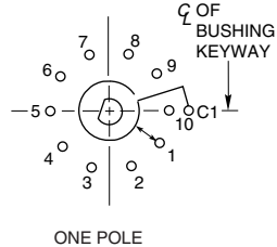
ONE POLE
