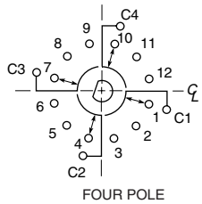
FOUR POLE
