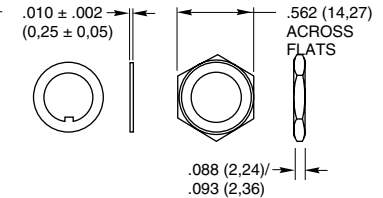
Keyed Washer
