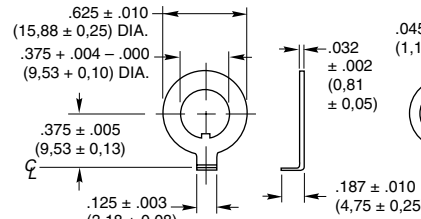
Non-Turn Washer
