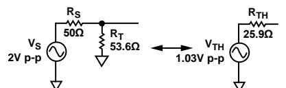
Figure 61. Calculating the Thevenin Equivalent
