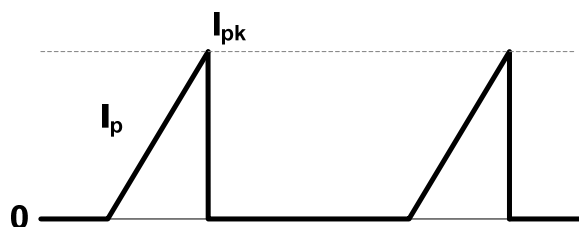
Figure 4: Primary Current Waveform
