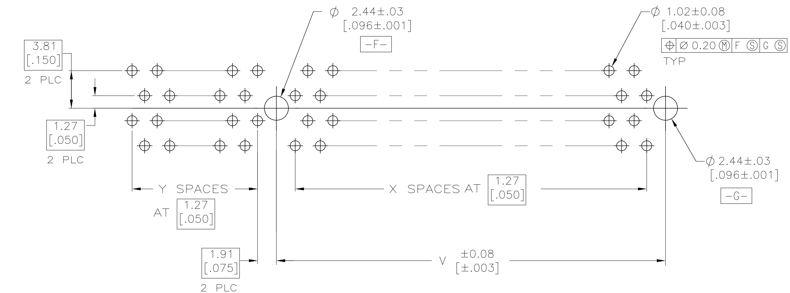
RECOMMENDED CONNECTOR MOUNTING HOLE PATTERN A (CONNECTOR SIDE SHOWN)
