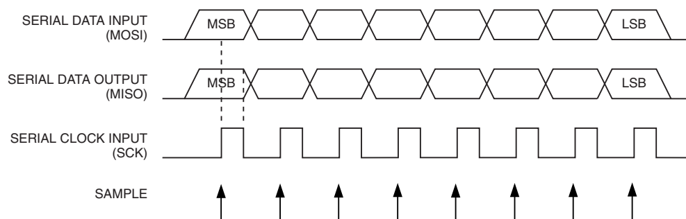
Figure 6-126. Serial Programming Waveforms
