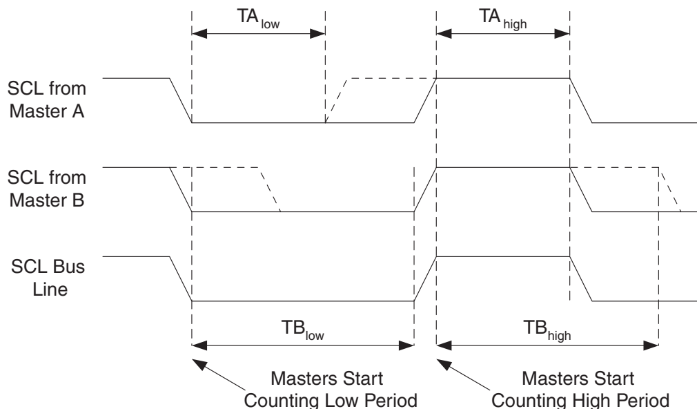
Figure 6-83. SCL Synchronization Between Multiple Masters
