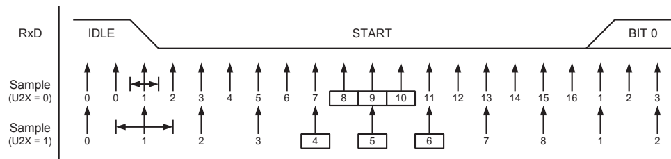
Figure 6-73. Start Bit Sampling
