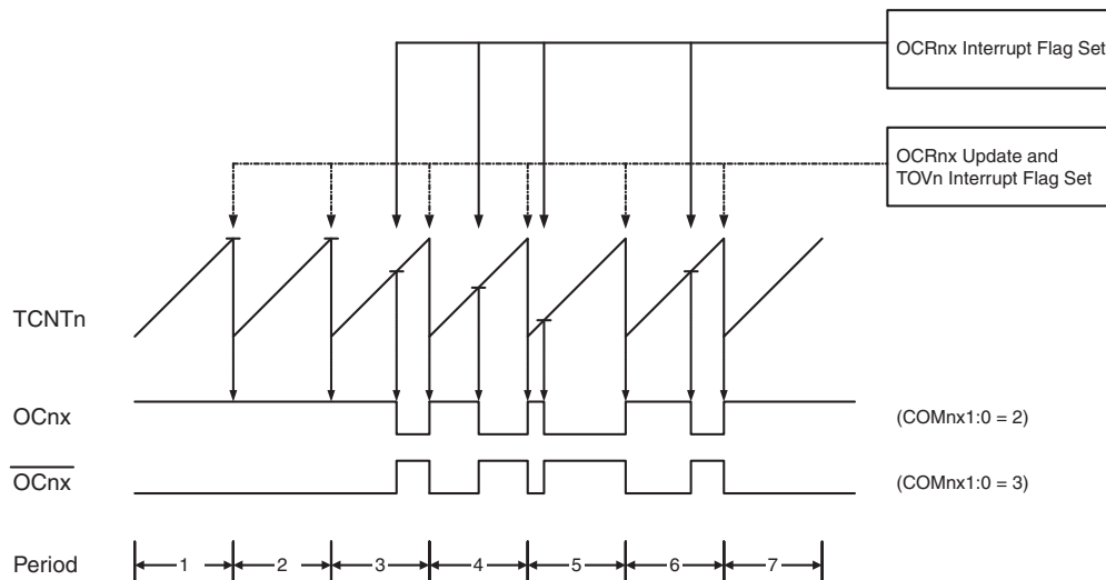
Figure 6-32. Fast PWM Mode, Timing Diagram
