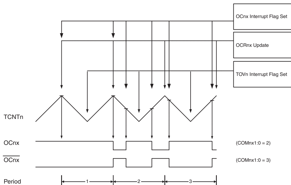
Figure 6-59. Phase Correct PWM Mode, Timing Diagram
