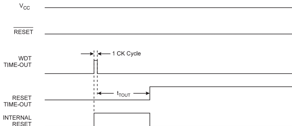
Figure 6-19. Watchdog System Reset During Operation
