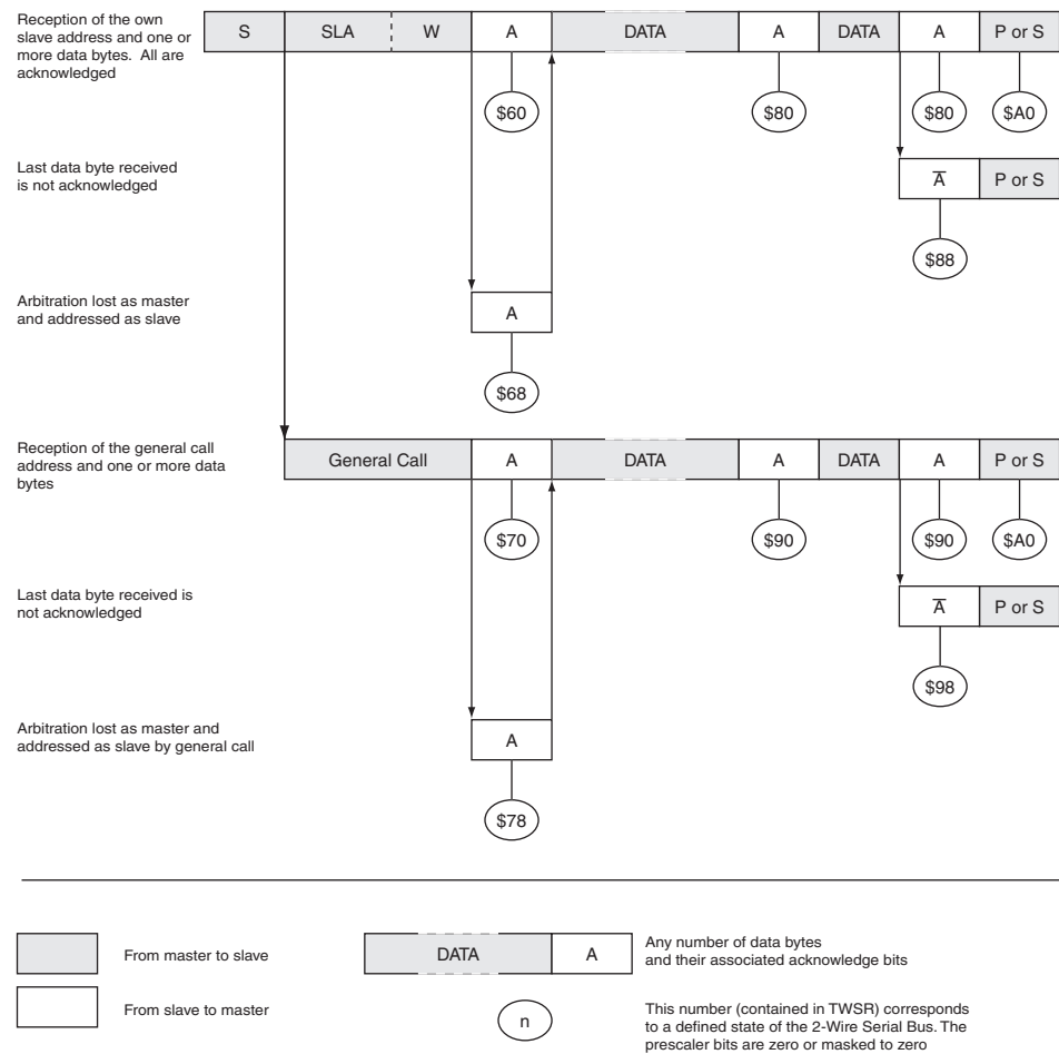
Figure 6-92. Formats and States in the Slave Receiver Mode
