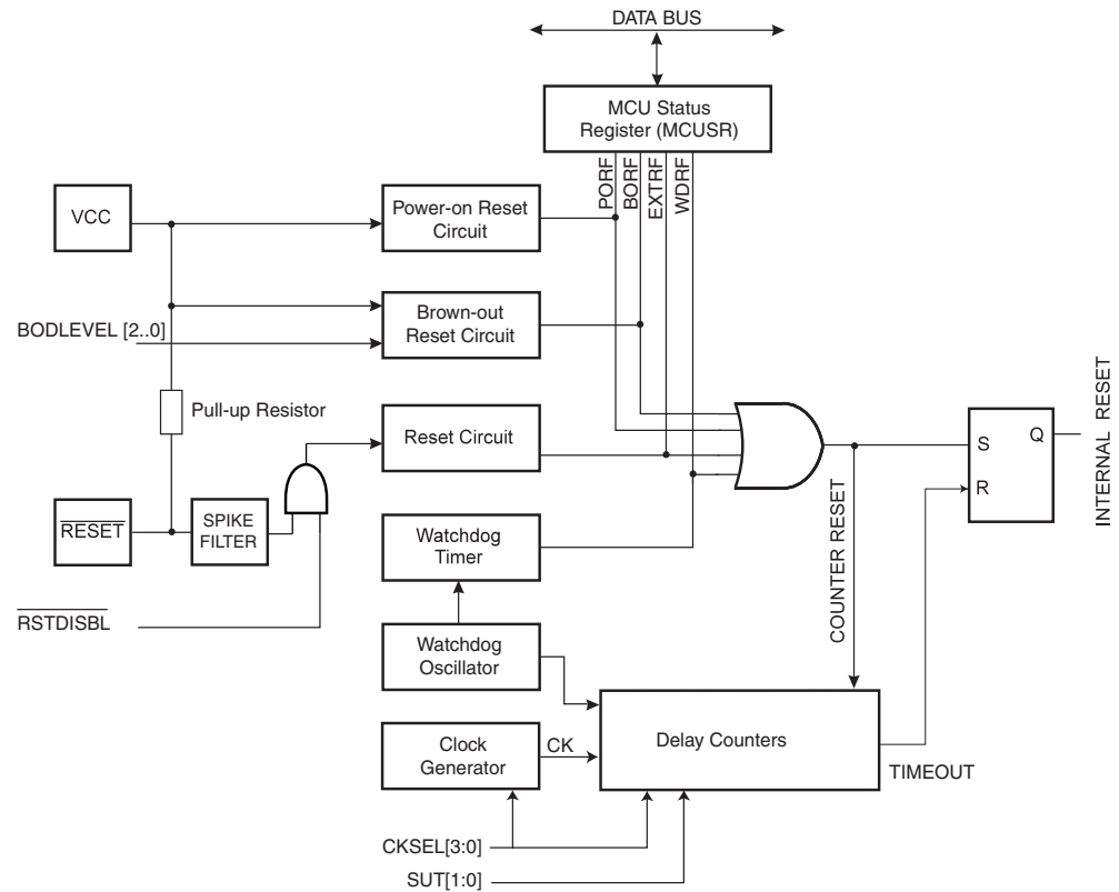
Figure 6-14. Reset Logic
