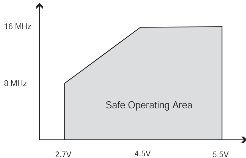
Figure 6-127. Maximum Frequency
