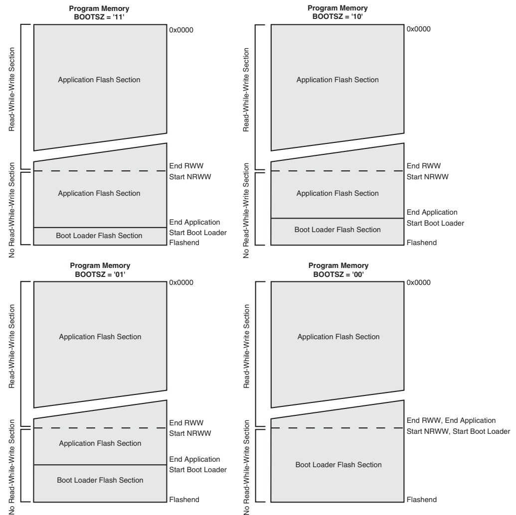
Figure 6-116. Memory Sections
