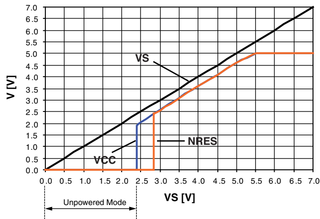
Figure 3-9. VCC and NRES versus VS (Ramp Up)
