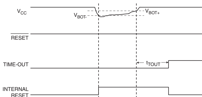
Figure 6-18. Brown-out Reset During Operation
