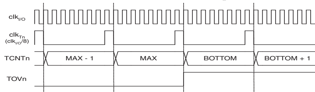
Figure 6-61. Timer/Counter Timing Diagram, with Prescaler ( f_{\text{clk}_{I/O}}/8 )
