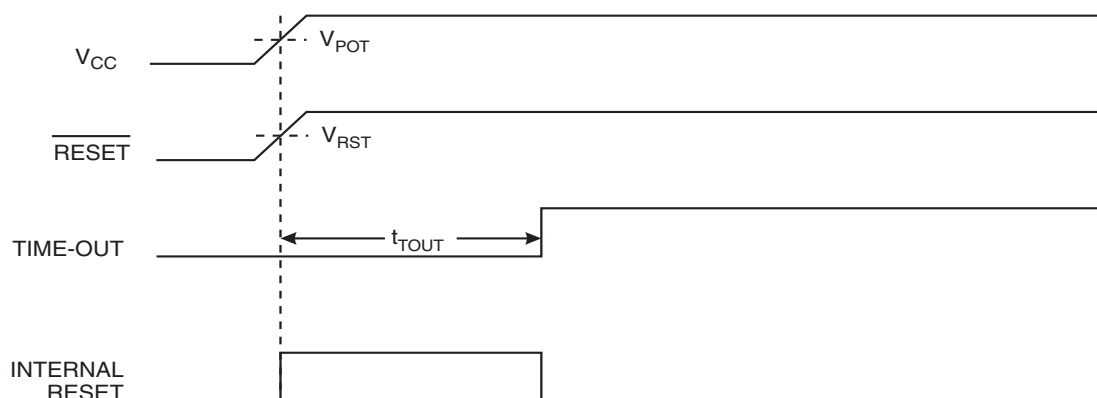
Figure 6-15. MCU Start-up, \overline{\text{RESET}} Tied to V_{CC}
