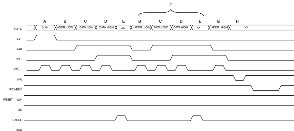
Figure 6-120. Programming the Flash Waveforms (1)
