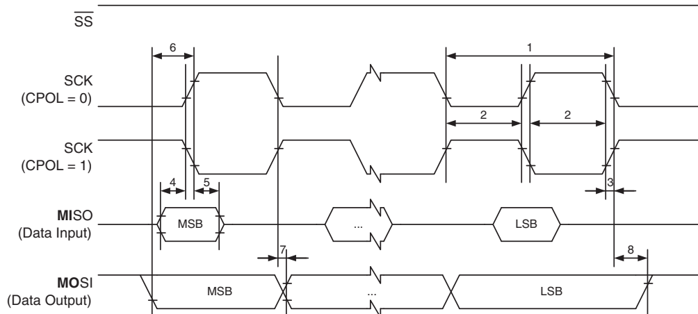
Figure 6-129. SPI Interface Timing Requirements (Master Mode)
