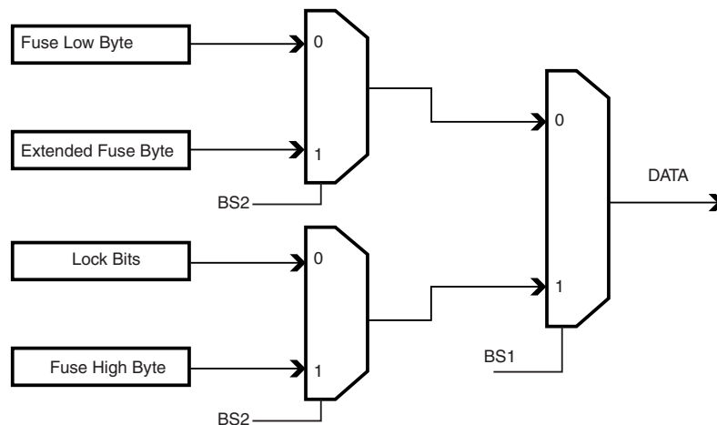
Figure 6-123. Mapping Between BS1, BS2 and the Fuse and Lock Bits During Read
