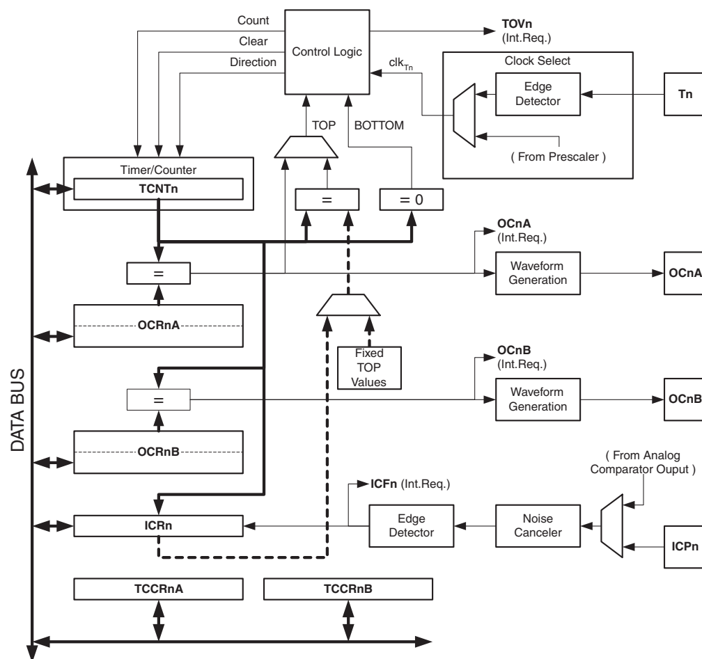
Figure 6-38. 16-bit Timer/Counter Block Diagram (1)
