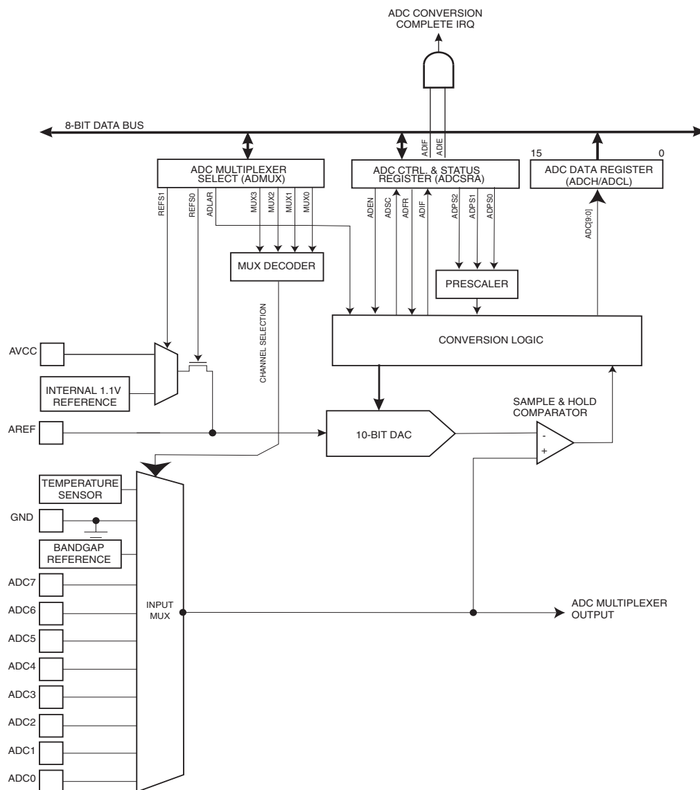
ABC CONVERSION
