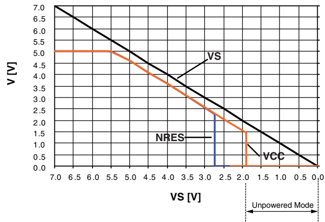
Figure 3-10. VCC and NRES versus VS (Ramp Down)
