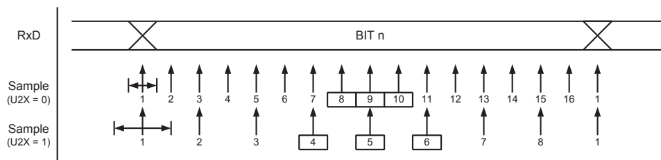
Figure 6-74. Sampling of Data and Parity Bit
