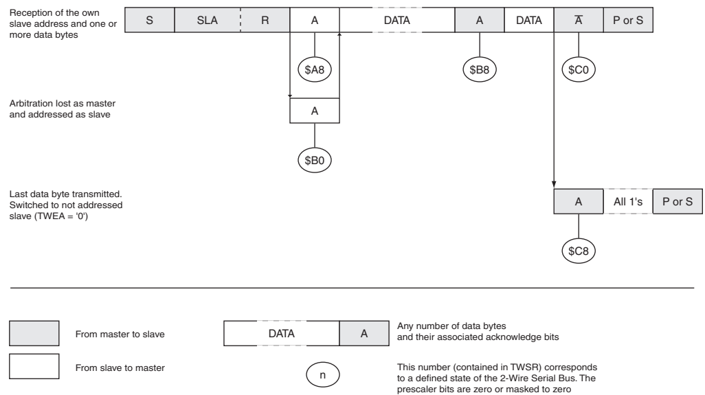
Figure 6-94. Formats and States in the Slave Transmitter Mode
