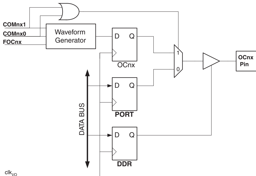
Figure 6-42. Compare Match Output Unit, Schematic
