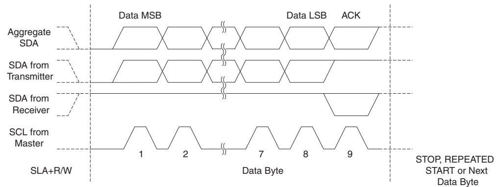
Figure 6-81. Data Packet Format
