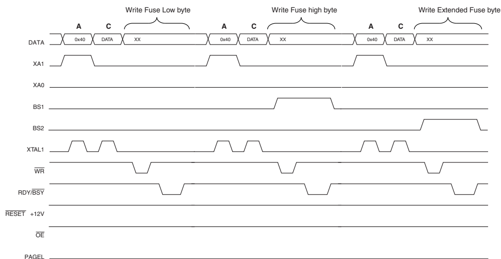
Figure 6-122. Programming the FUSES Waveforms
