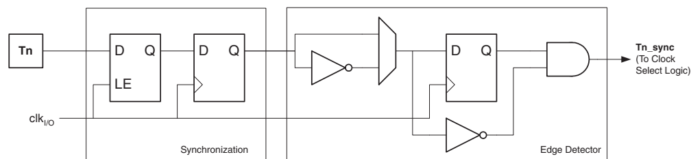
Figure 6-51. T1/T0 Pin Sampling
