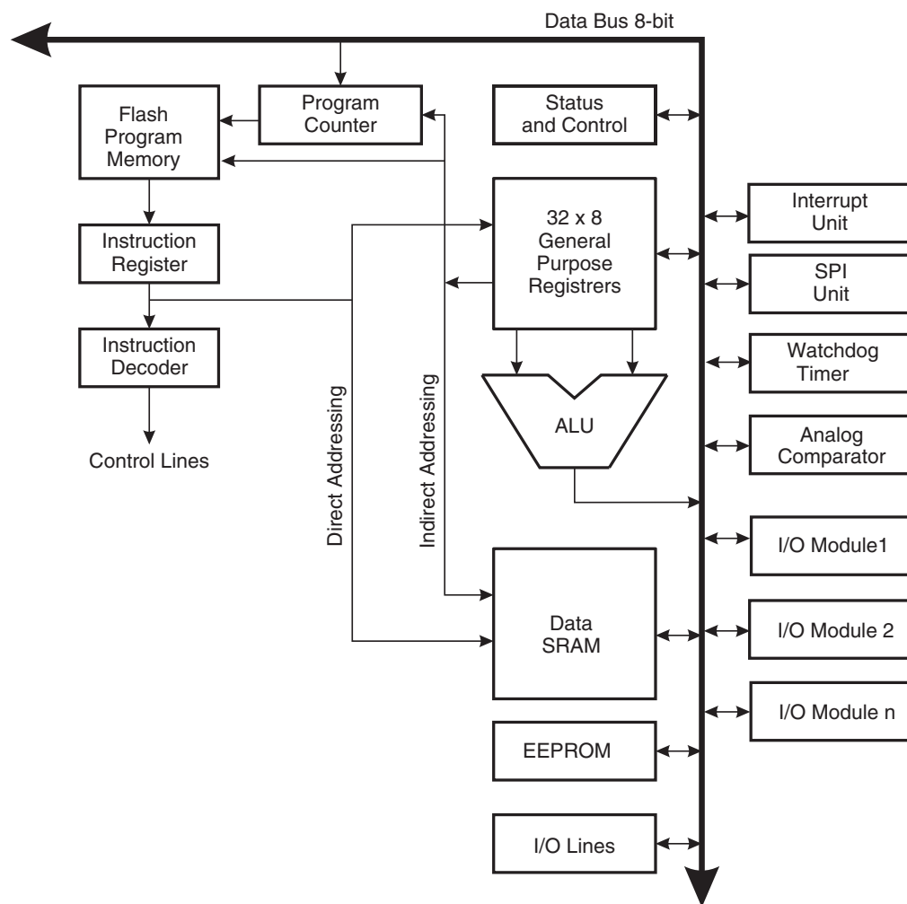
Figure 6-2. Block Diagram of the AVR Architecture
