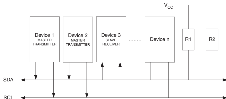
Figure 6-96. An Arbitration Example
