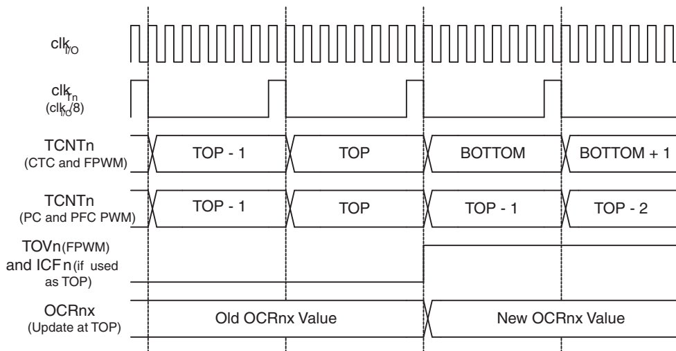
Figure 6-50. Timer/Counter Timing Diagram, with Prescaler ( f_{clk\_I/O}/8 )
