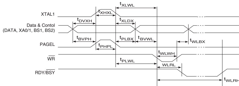
Figure 6-132. Parallel Programming Timing, Including some General Timing Requirements
