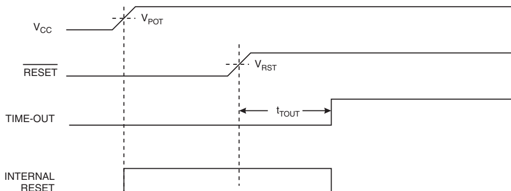
Figure 6-16. MCU Start-up, \overline{\text{RESET}} Extended Externally
