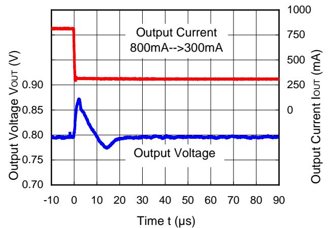
RP505K081A/B ( V_{IN}=3.6V )
