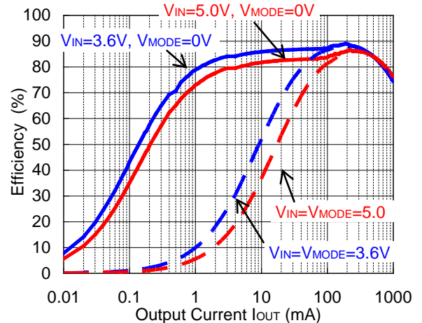
RP505K V OUT =3.3V
