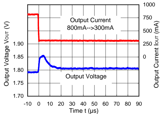
RP505K181A/B ( V_{IN}=3.6V )
