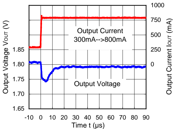
RP505K181A/B ( V_{IN}=3.6V )
