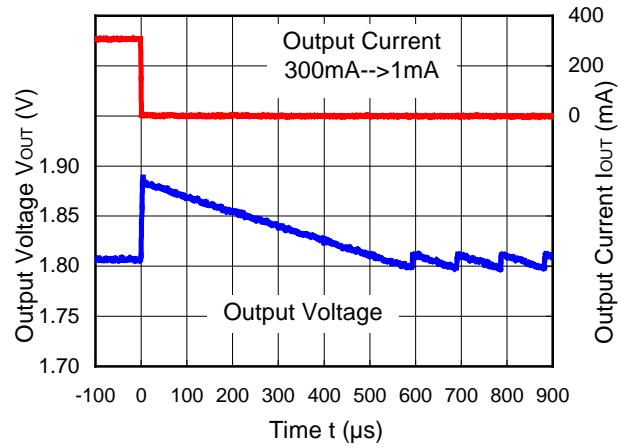
RP505K181A/B ( V_{IN}=3.6V ) MODE="L" PWM/VFM automatic shift
