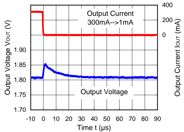
RP505K001C ( V_{IN}=3.6V , V_{OUT}=1.8V ) MODE="H" forced PWM
