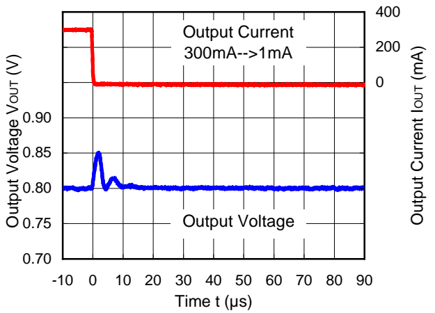
RP505K001C (V IN =3.6V, V OUT =0.8V) MODE="H" forced PWM
