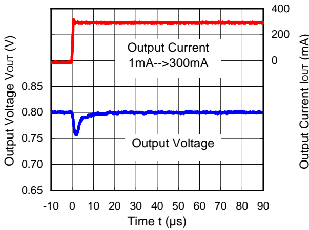
RP505K001C (V IN =3.6V, V OUT =0.8V) MODE="H" forced PWM
