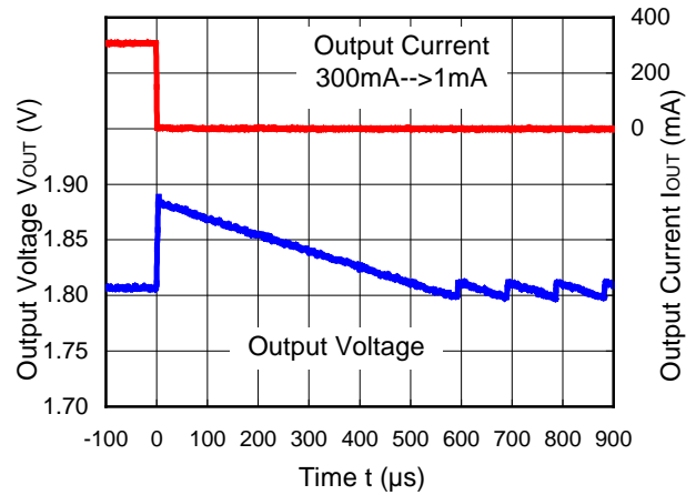
RP505K181A/B ( V_{IN}=3.6V ) MODE="L" PWM/VFM automatic shift
