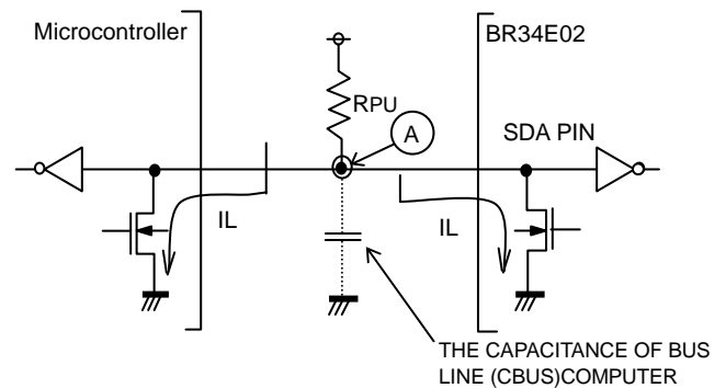
Fig.43 I/O Circuit
