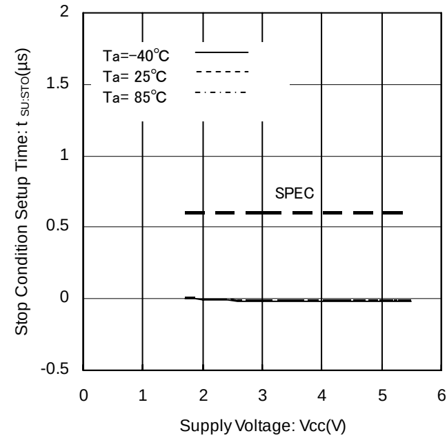
Figure 24. Stop Condition Setup Time vs Supply Voltage
