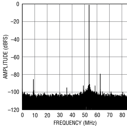
LTC2150-12: 32K Point FFT, f_{IN} = 225\text{MHz} , -1\text{dBFS} , 170Msps
