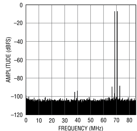
LTC2150-12: 32K Point 2-Tone FFT, f_{IN} = 71\text{MHz} and 69\text{MHz} , 170Msps
