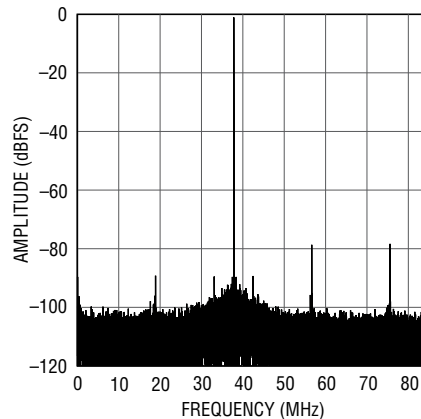
LTC2150-12: 32K Point FFT, f_{IN} = 380\text{MHz} , -1\text{dBFS} , 170Msps
