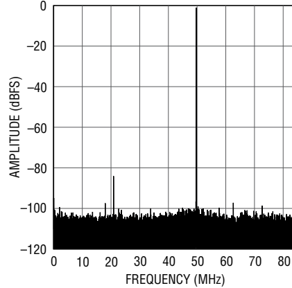
LTC2150-12: 32K Point FFT, f_{IN} = 121\text{MHz} , -1\text{dBFS} , 170Msps
