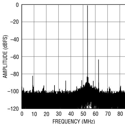
LTC2150-12: 32K Point FFT, f_{IN} = 567\text{MHz} , -1\text{dBFS} , 170Msps
