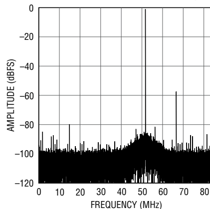
LTC2150-12: 32K Point FFT, f_{IN} = 907\text{MHz} , -1\text{dBFS} , 170Msps
