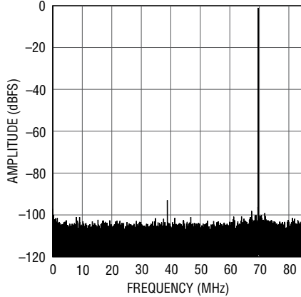
LTC2150-12: 32K Point FFT, f_{IN} = 70\text{MHz} , -1\text{dBFS} , 170Msps
