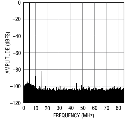
LTC2150-12: 32K Point FFT, f_{IN} = 176\text{MHz} , -1\text{dBFS} , 170Msps
