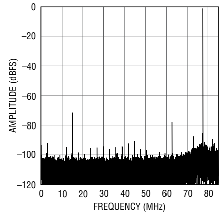
LTC2150-12: 32K Point FFT, f_{IN} = 420\text{MHz} , -1\text{dBFS} , 170Msps
