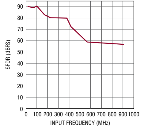
LTC2151-12: SFDR vs Input Level, -1dBFS, 1.5V Range, 210Msps
