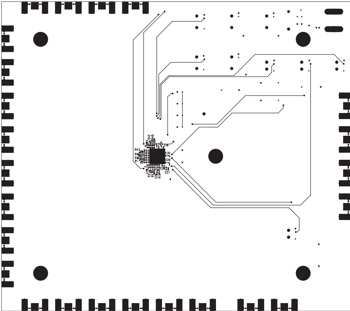
Figure 7. MAX3678 EV Kit Component Placement Guide—Solder Side
