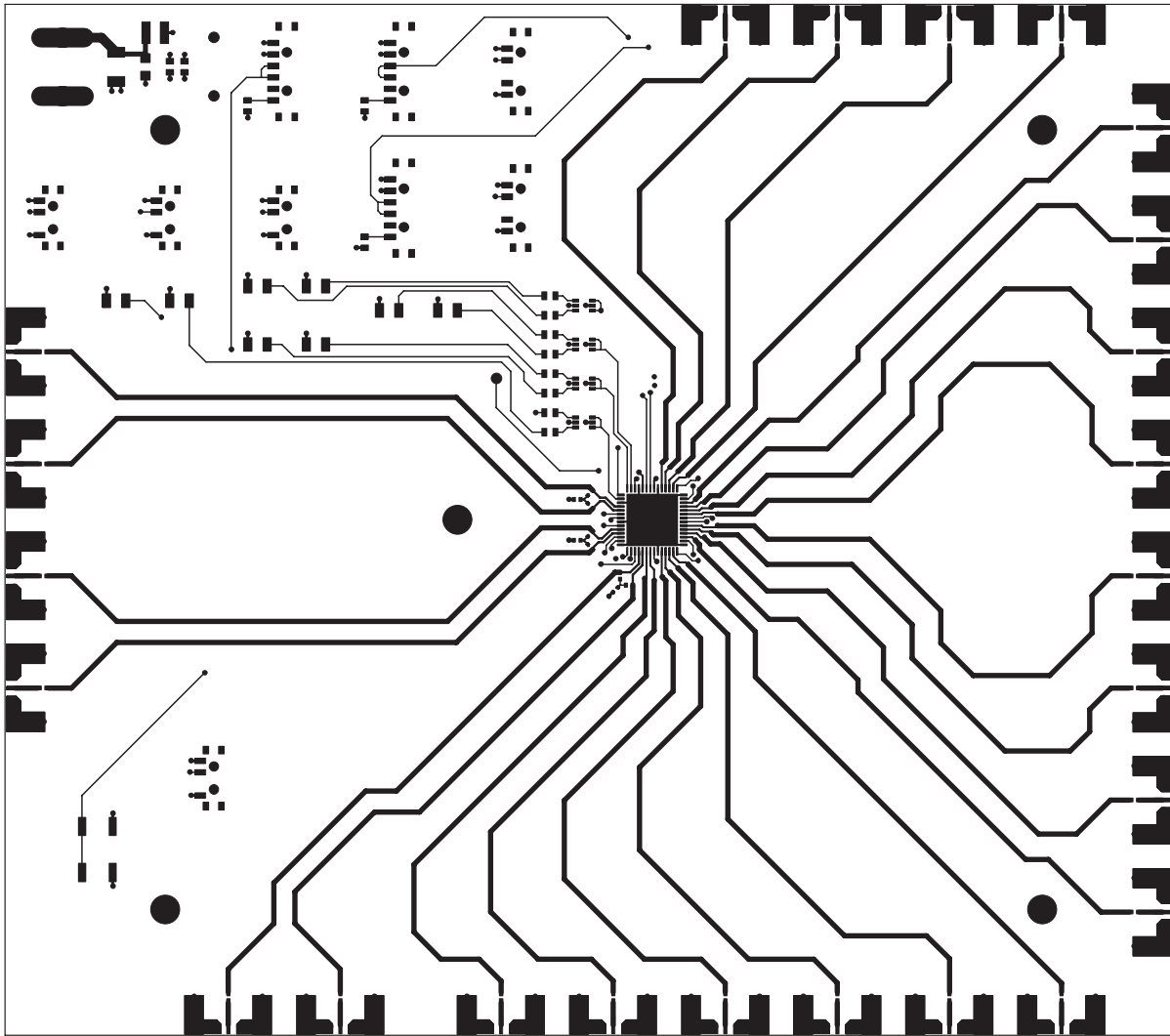
Figure 3. MAX3678 EV Kit PCB Layout—Component Side
