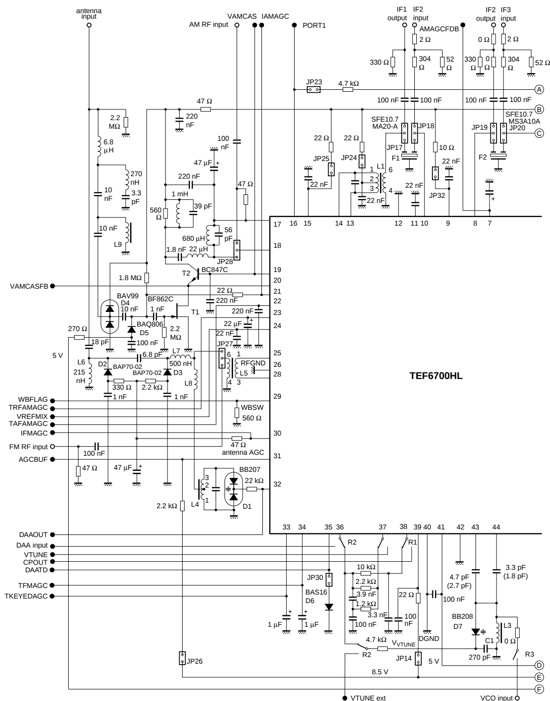
Fig.8 Test circuit (continued in Fig.9).
