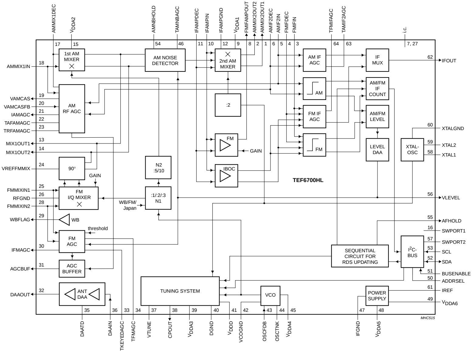
Fig.1 Block diagram.
