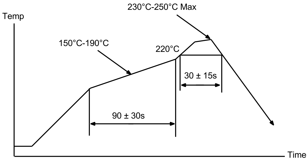
Figure 8 - Reflow Profile for Lead Free Solder
