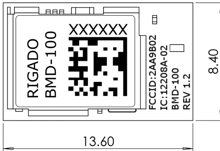
Figure 6 – Module Marking – Rev A
