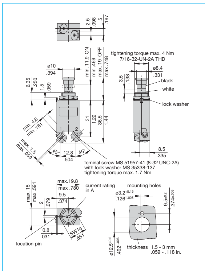
Dimensions 483-G533-J1M1-B2S0ZN (MS 3320)
