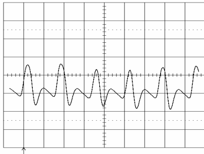
Output voltage ripple (20mV/div.) at: T_{ref} = +25^{\circ}\text{C} , I_O = 10\text{ A} resistive load, V_I = 5.0\text{ V} . Time scale: 2 \mu\text{s} /div. See the filter in the Output ripple and noise section (EMC Specification).
