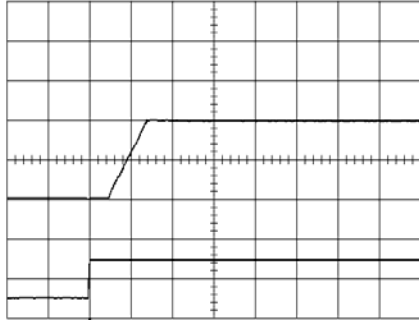
Start-up enabled by connecting V_I at: T_{ref} = +25^{\circ}\text{C} , I_O = 10\text{ A} resistive load, V_I = 5.0\text{ V} . Top trace: output voltage (0.5 V/div.). Bottom trace: input voltage (5 V/div.). Time scale: 5 ms/div..
