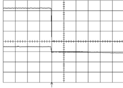
Shut-down enabled by disconnecting V_i at: T_{ref} = +25^\circ\text{C} , I_O = 10\text{ A} resistive load, V_i = 5.0\text{ V} . Top trace: output voltage (1.0 V/div.). Bottom trace: input voltage (2 V/div.). Time scale: 5.0 ms/div..
