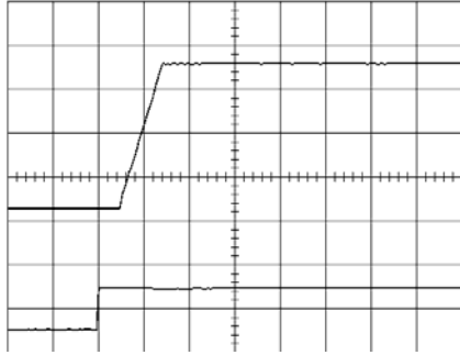
Start-up enabled by connecting V_i at: T_{ref} = +25^\circ\text{C} , I_O = 10\text{ A} resistive load, V_i = 5.0\text{ V} . Top trace: output voltage (1.0 V/div.). Bottom trace: input voltage (5 V/div.). Time scale: 5 ms/div..
