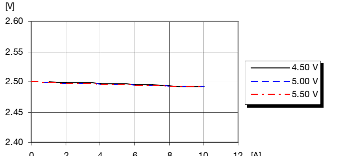
Output voltage vs. load current at T_{ref} = +25^{\circ}C
