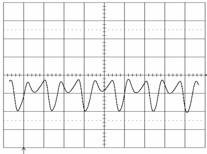
Output voltage ripple (20mV/div.) at: T_{ref} = +25^\circ\text{C} , I_O = 10\text{ A} resistive load, V_i = 5.0\text{ V} . Time scale: 2 \mu\text{s} /div. See the filter in the Output ripple and noise section (EMC Specification).
