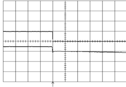
Shut-down enabled by disconnecting V_I at: T_{ref} = +25^{\circ}\text{C} , I_O = 10\text{ A} resistive load, V_I = 5.0\text{ V} . Top trace: output voltage (1.0 V/div.). Bottom trace: input voltage (2 V/div.). Time scale: 5.0 ms/div..
