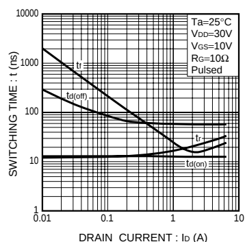
Fig.7 Switching Characteristics
