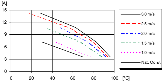
Available load current vs. ambient air temperature and airflow at V_I = 27 V. See Thermal Consideration section.
