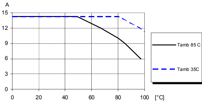
Available load current vs. base plate temperature. V_I = 27 V. See Thermal Consideration section.
