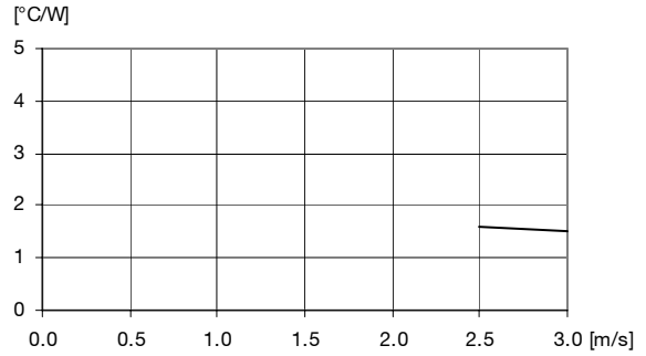
Thermal resistance vs. airspeed measured at the converter. Tested in wind tunnel with airflow and test conditions as per the Thermal consideration section. V_I = 27 V.
