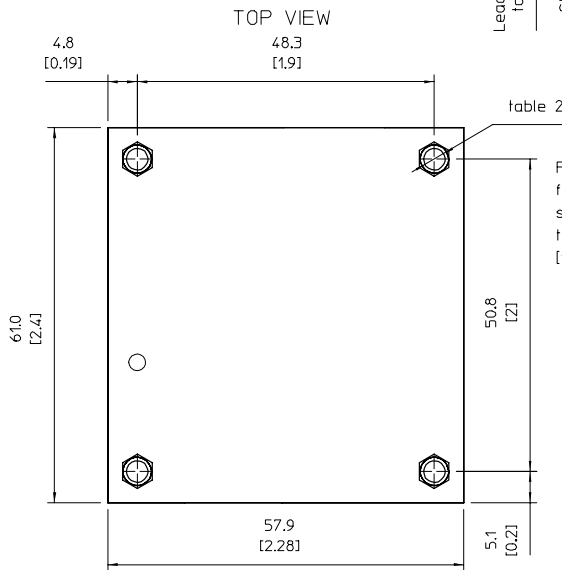
Recommended Footprint - TOP VIEW
