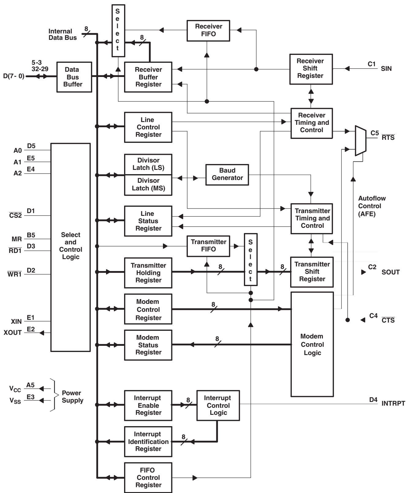
FUNCTIONAL BLOCK DIAGRAM (For ZQS Package)
