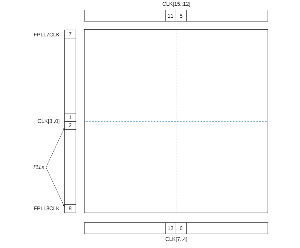
Figure 2–70. PLL Locations
