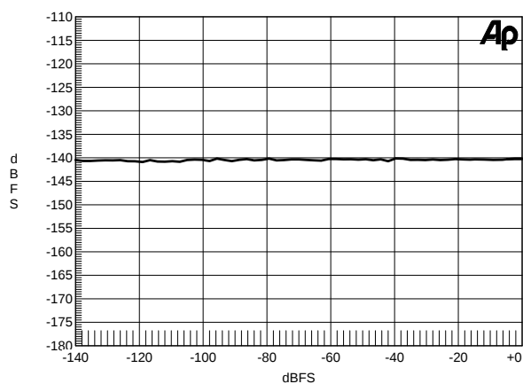
Figure 57. THD+N vs. Input Amplitude, 1 kHz Tone,
