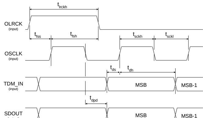
Figure 2. TDM Slave Mode Timing
