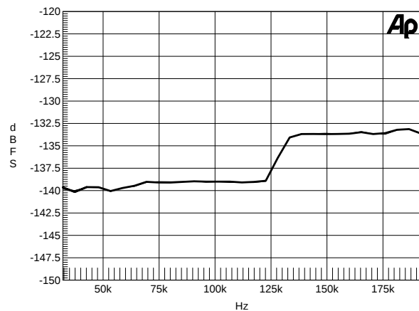
Figure 43. THD+N vs. Output Sample Rate, 0 dBFS
