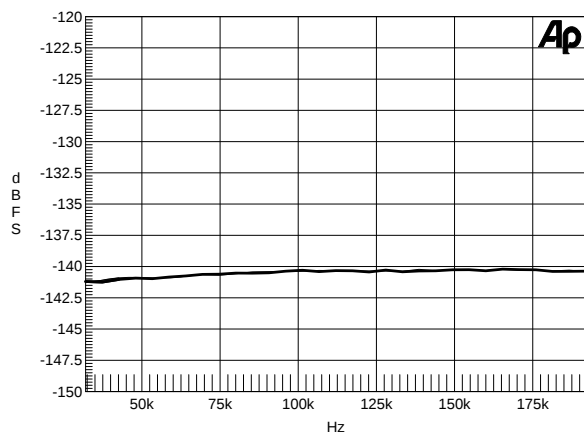
Figure 45. Dynamic Range vs. Output Sample Rate,
