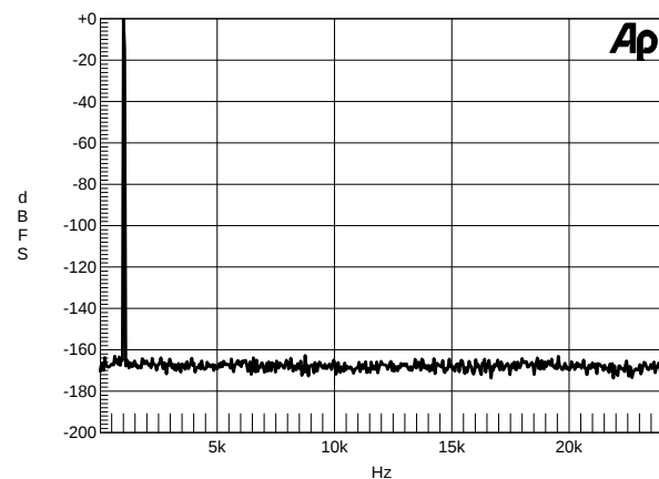
Figure 17. Wideband FFT Plot (16k Points) 0 dBFS
