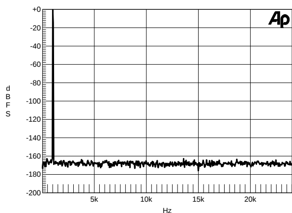
Figure 15. Wideband FFT Plot (16k Points) 0 dBFS
