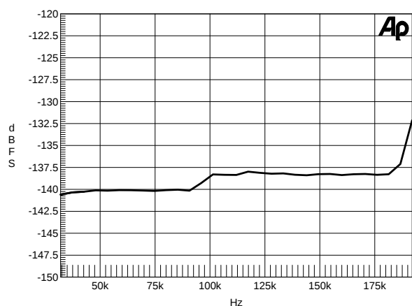
Figure 39. THD+N vs. Output Sample Rate, 0 dBFS
