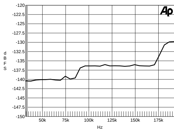
Figure 41. THD+N vs. Output Sample Rate, 0 dBFS
