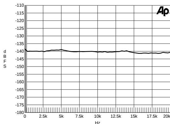
Figure 65. THD+N vs. Frequency Input, 0 dBFS,
