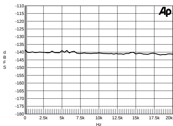
Figure 63. THD+N vs. Frequency Input, 0 dBFS,
