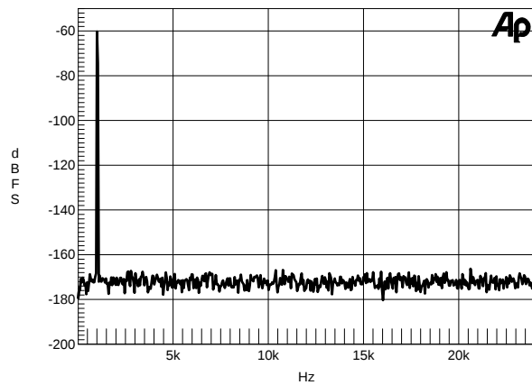
Figure 27. Wideband FFT Plot (16k Points) -
