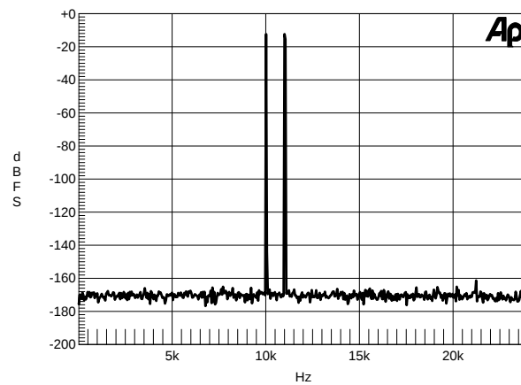
Figure 31. IMD, 10 kHz and 11 kHz -7 dBFS,
