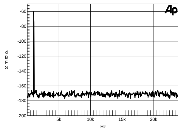
Figure 23. Wideband FFT Plot (16k Points) -
