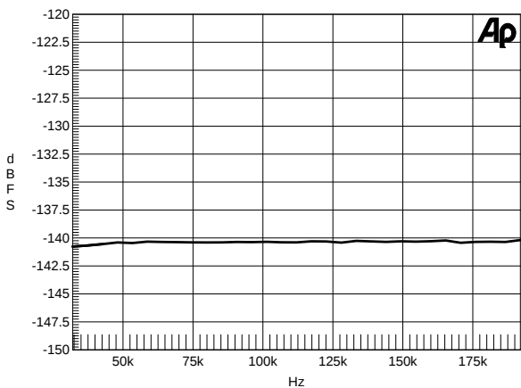
Figure 49. Dynamic Range vs. Output Sample Rate,
