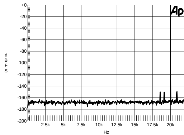
Figure 37. Wideband FFT Plot (16k Points) 0 dBFS
