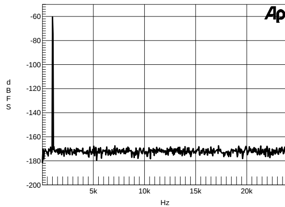
Figure 29. Wideband FFT Plot (16k Points) -
