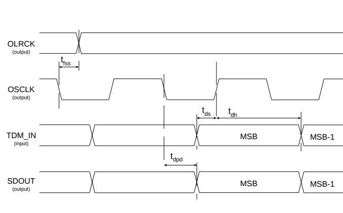
Figure 4. TDM Master Mode Timing
