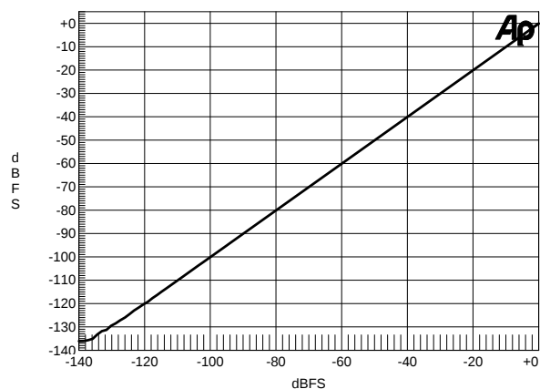
Figure 51. Linearity Error, 0 to -140 dBFS Input,
