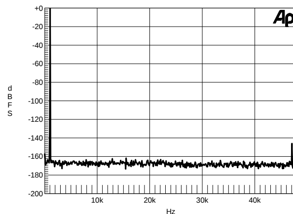
Figure 19. Wideband FFT Plot (16k Points) 0 dBFS
