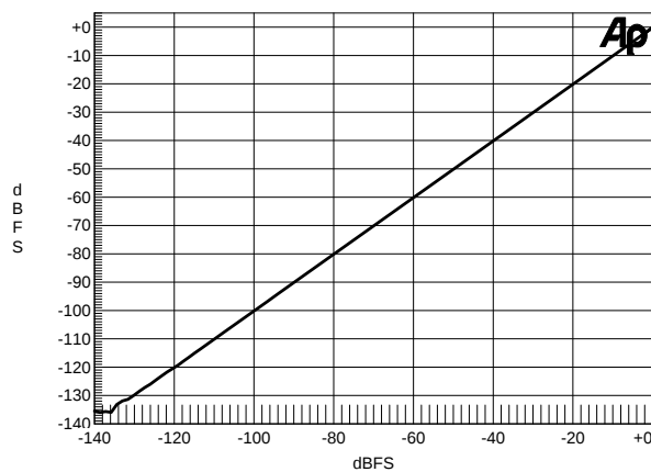
Figure 55. Linearity Error, 0 to -140 dBFS Input,
