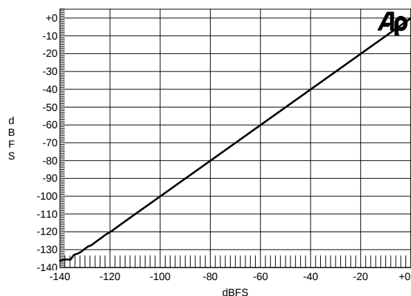
Figure 53. Linearity Error, 0 to -140 dBFS Input,
