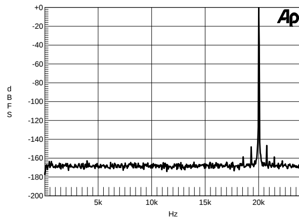
Figure 35. Wideband FFT Plot (16k Points) 0 dBFS
