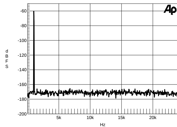
Figure 25. Wideband FFT Plot (16k Points) -
