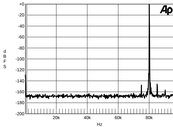
Figure 33. Wideband FFT Plot (16k Points) 0 dBFS
