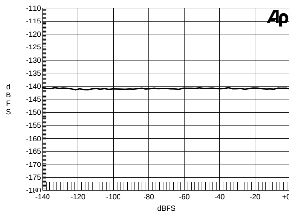
Figure 59. THD+N vs. Input Amplitude, 1 kHz Tone,
