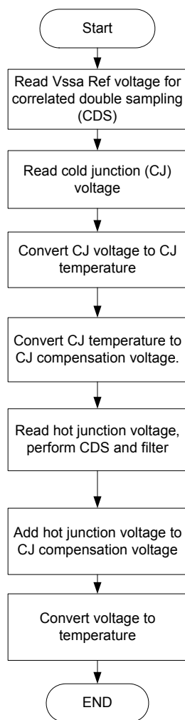
Figure 5-6. Thermocouple Flowchart
