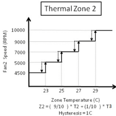
Figure 5-33. Thermal Management System Project - Zone2 Thermal Profile
