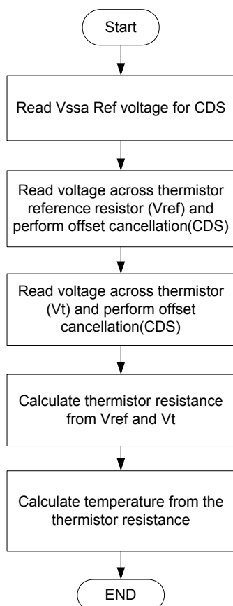
Figure 5-7. Thermistor Flowchart
