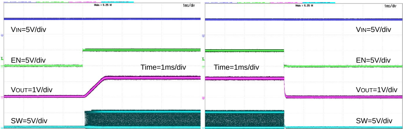
Figure 29. Power Down Waveform with EN (FREQ=H, R LOAD =0.5Ω)
