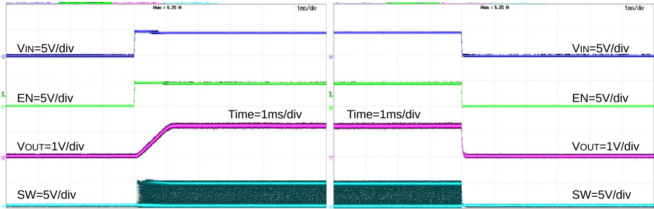
Figure 31. Power Down Waveform with V IN (FREQ=H, R LOAD =0.5Ω)
