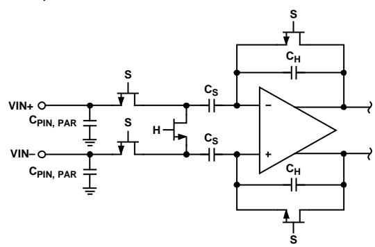
Figure 45. Switched-Capacitor SHA Input
