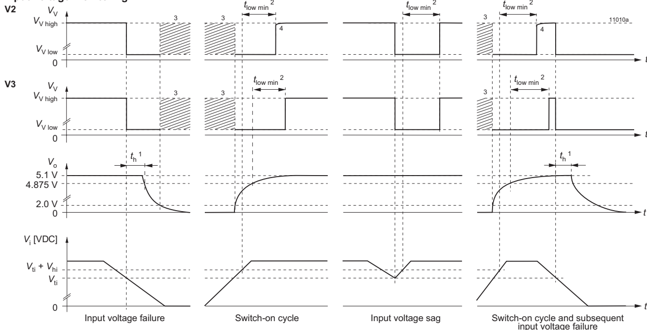
Fig. 40 Output configuration of options V0, V2 and V3
