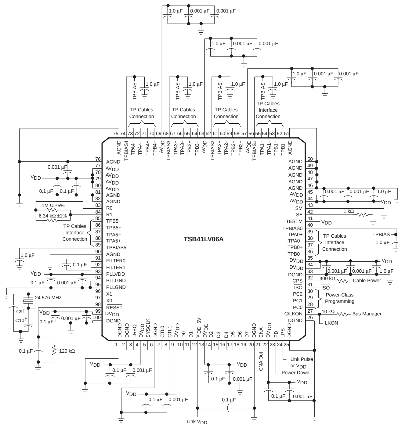
Figure 9. External Component Connections
