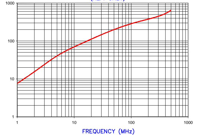
AGILENT E4991A Impedance/Material Analyzer HP 16092A-Test Fixture, REF 3158
