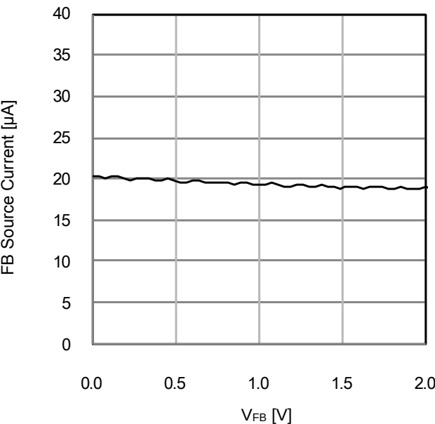
Figure 8. FB Source Current vs V_{FB} ( V_{INV}=0.2\text{V} , V_{FB}=1.5\text{V} )
