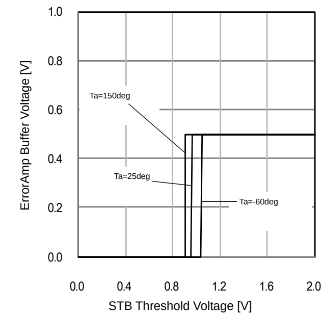
Figure 9. ErrorAmp Buffer Voltage vs STB Threshold Voltage
