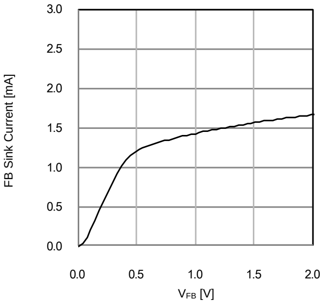
Figure 7. FB Sink Current vs V_{FB} ( V_{INV}=0.8\text{V} , V_{FB}=1.5\text{V} )
