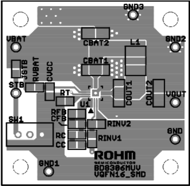
Figure 20. Assembly Layer
