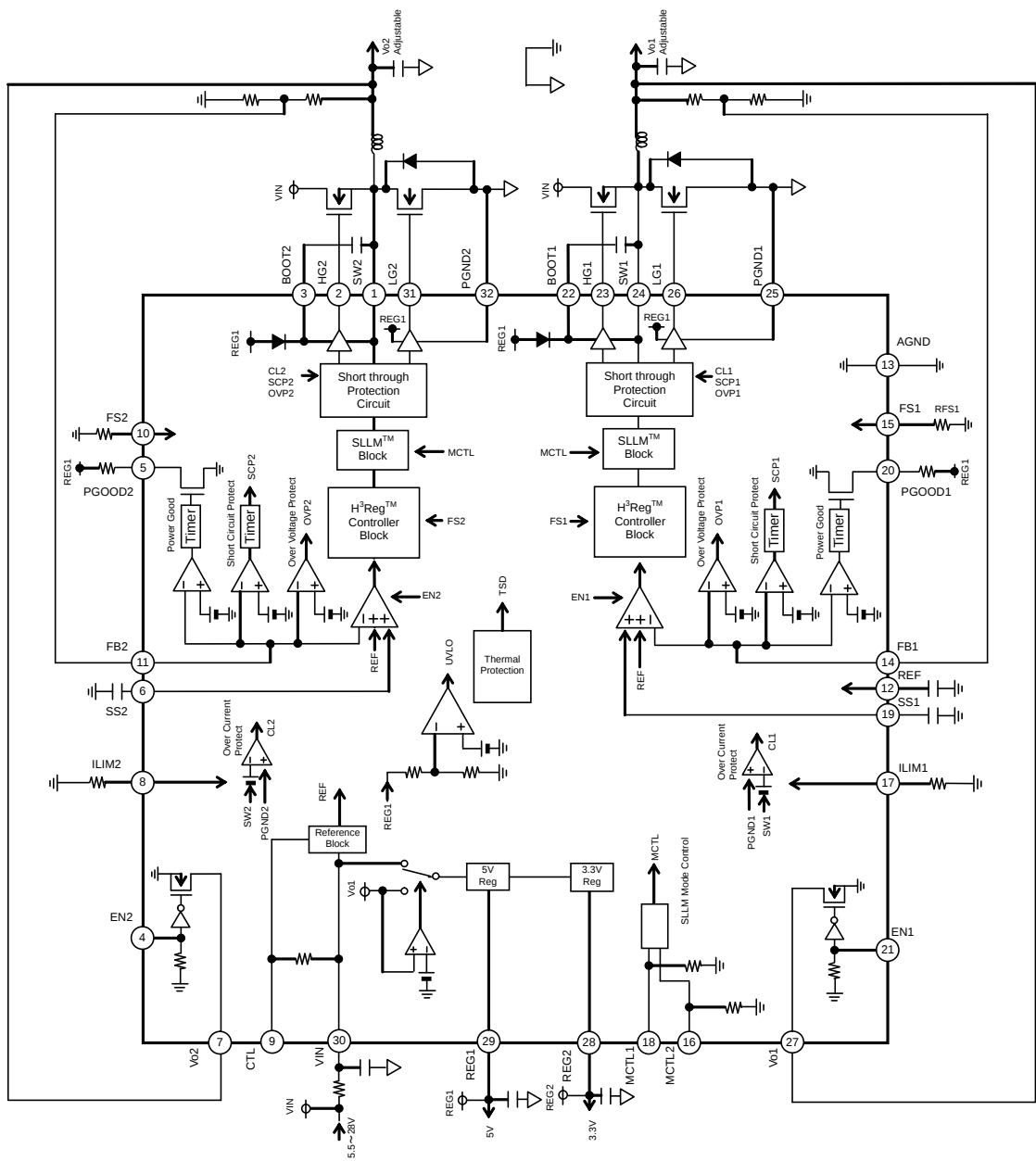
Block Diagram
