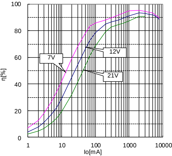
Figure 20. Efficiency (Vo= 3.3V, QLLM)
