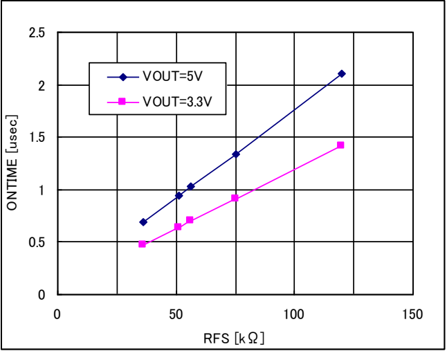
Figure 49. On time-RFS
