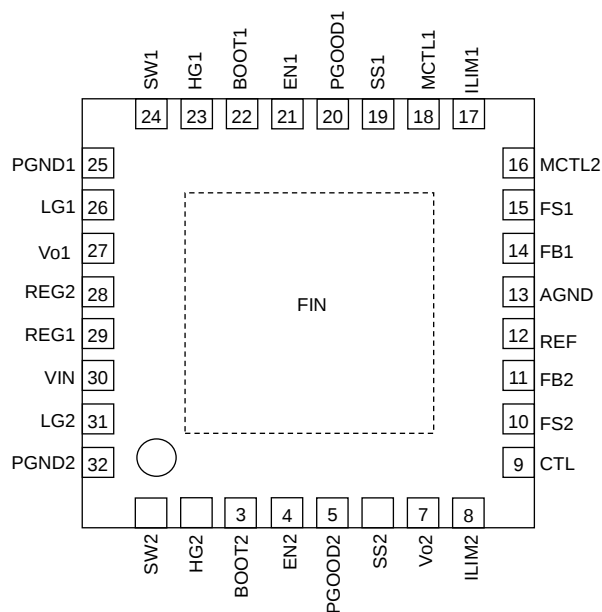
Figure 2. Pin Configuration
