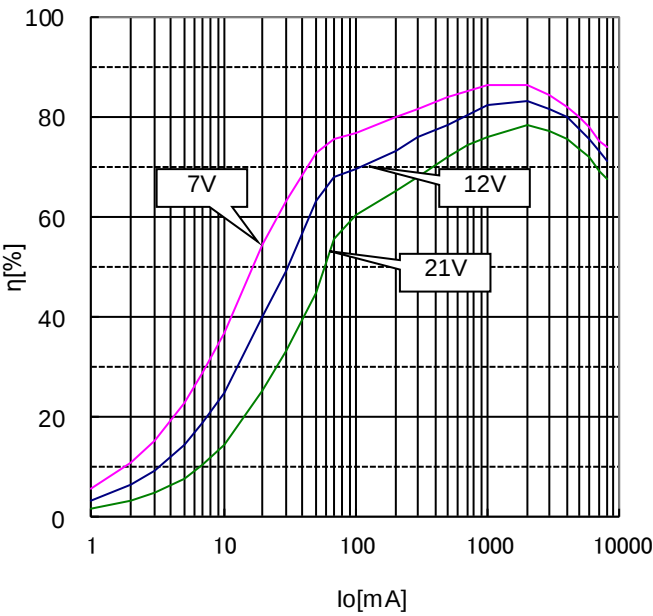
Figure 23. Efficiency (Vo= 1V, QLLM)
