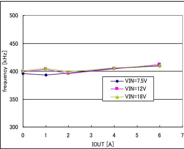
Figure 48. I o -frequency (V o = 3.3V, PWM, RFS= 68k \Omega )
