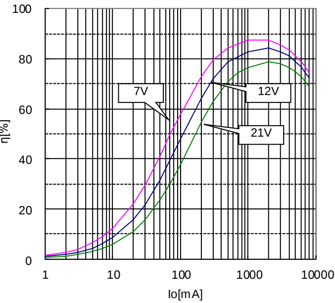
Figure 22. Efficiency (Vo= 1V, PWM)
