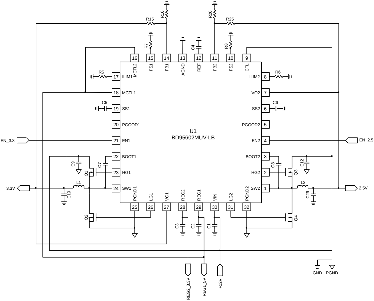
Figure 57. Application Example
