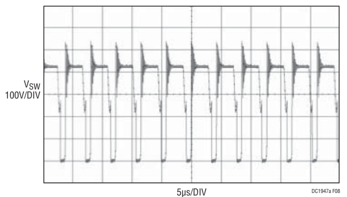
Figure 8. V_{IN} = 230VAC
