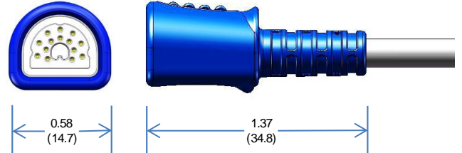
Cable-mount receptacle
