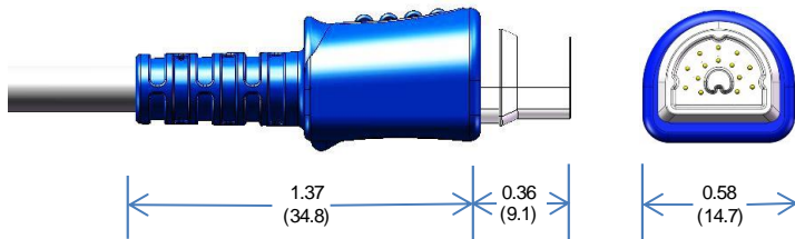
Cable-mount plug
