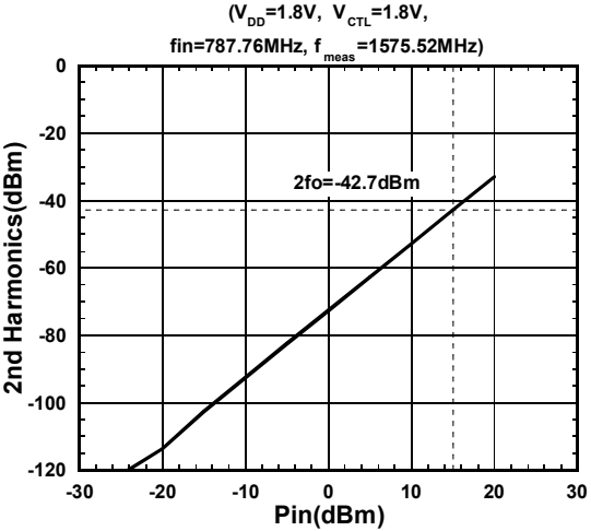
2nd Harmonics
