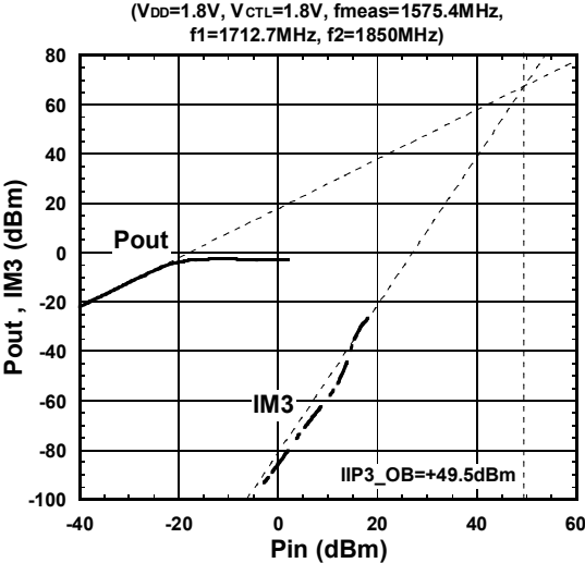
Out-of-band IIP3
