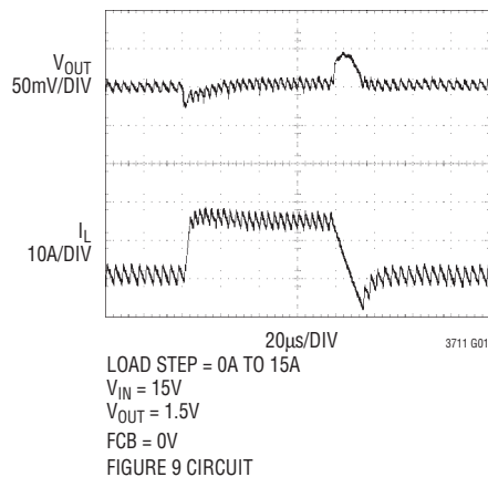
Transient Response
