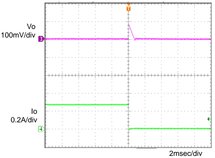
Figure 6. Transient Response (0.3→0A) Co=1 \mu F, Ta=-40°C
