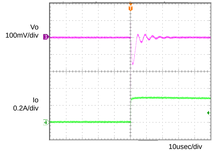
Figure 5. Transient Response (0→0.3A) Co=1μF, Ta=105°C
