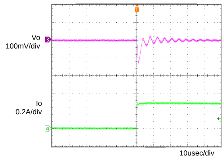
Figure 3. Transient Response (0→0.3A) Co=1μF, Ta=-40°C
