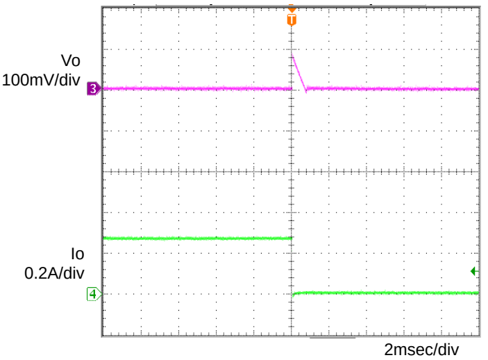
Figure 6. Transient Response (0.3→0A) Co=1μF, Ta=-40°C
