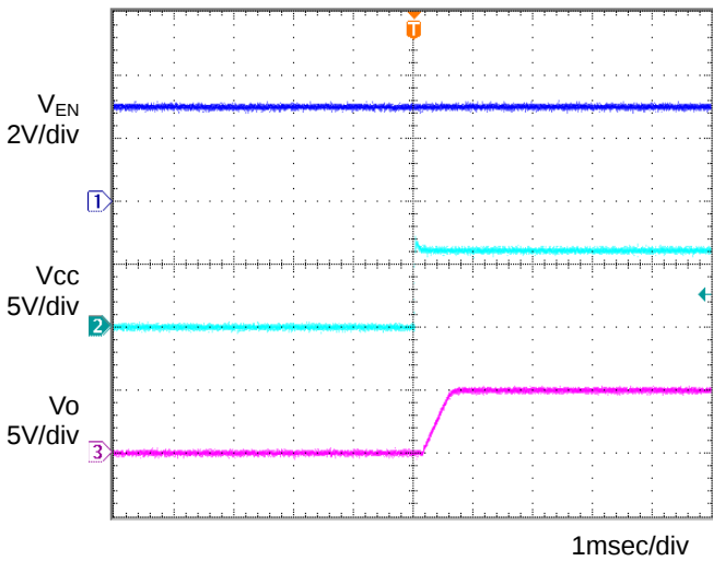
Figure 9. Input sequence 1 C_o = 1\mu\text{F} , T_a = -40^\circ\text{C}
