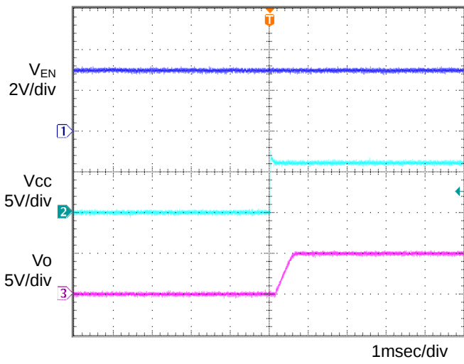
Figure 10. Input sequence 1 C_o = 1\mu\text{F} , T_a = 25^\circ\text{C}
