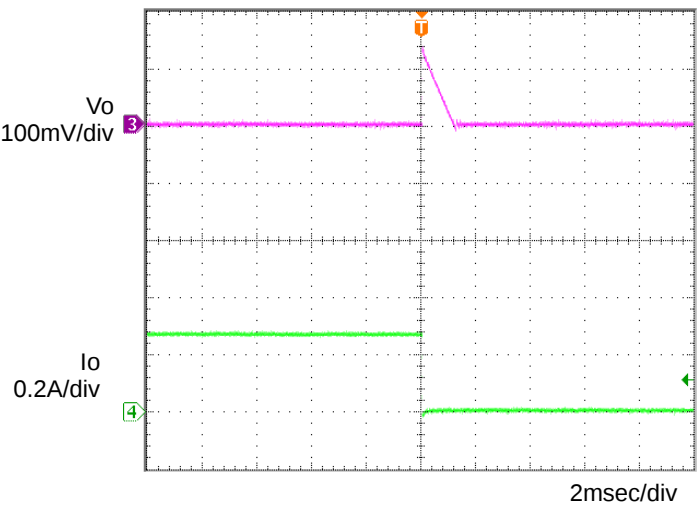
Figure 8. Transient Response (0.3→0A) C_o = 1\mu\text{F} , T_a = 105^\circ\text{C}
