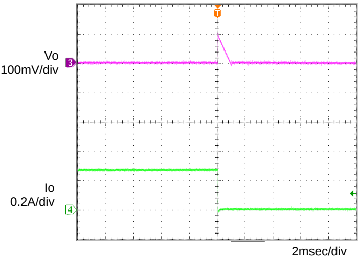
Figure 7. Transient Response (0.3→0A) C_o = 1\mu\text{F} , T_a = 25^\circ\text{C}
