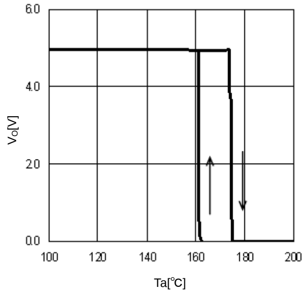
Figure 28. TSD ( I_o=0mA )
