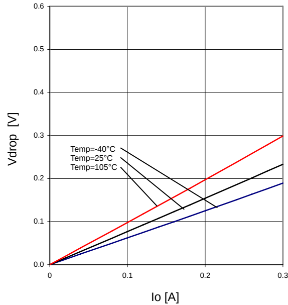
Figure 37. Minimum dropout Voltage 4 (V CC =10.0V)
